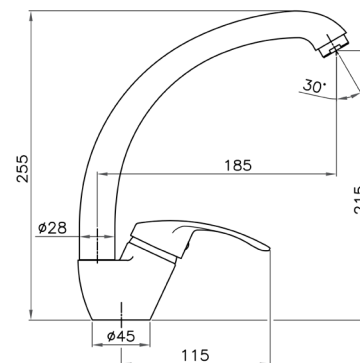
▲ Bathroom Faucet
