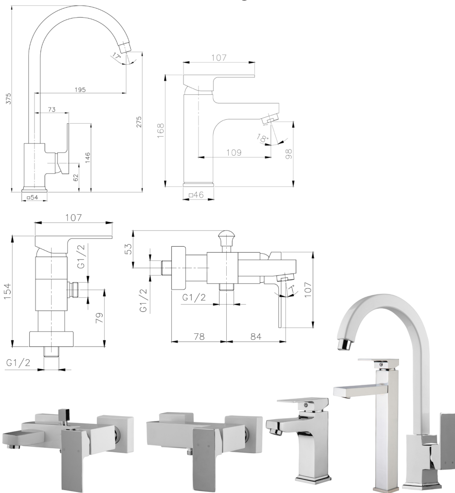
▲ Bathroom Faucet
