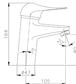
▲ Bathroom Faucet
